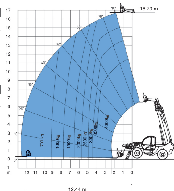
Lift capacity chart (with stabilisers)
